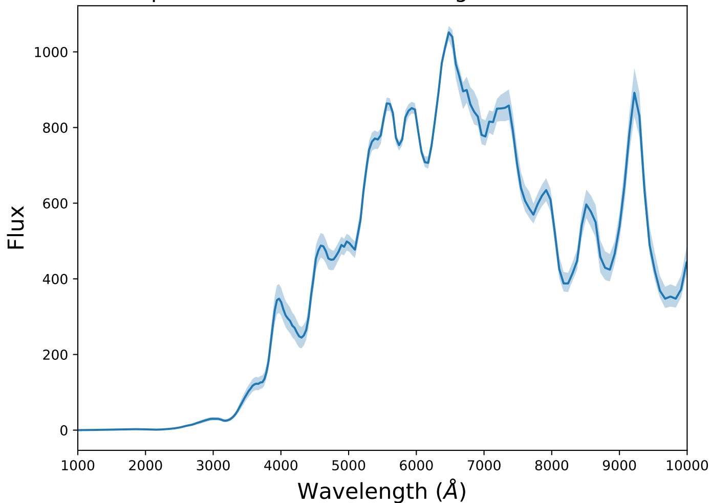
Spectrum 9 for transient 91bg-like at z=0.35
